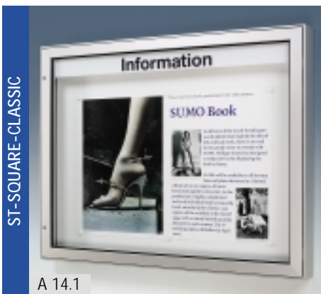
ST-SQUARE-CLASSIC Extruded aluminium profiles with mitred corners. 65mm deep with 65mm border on glass frontage.
