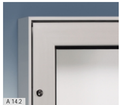
ST-SQUARE-CLASSIC Extruded aluminium profiles with mitred corners. 65mm deep with 65mm border on glass frontage.
